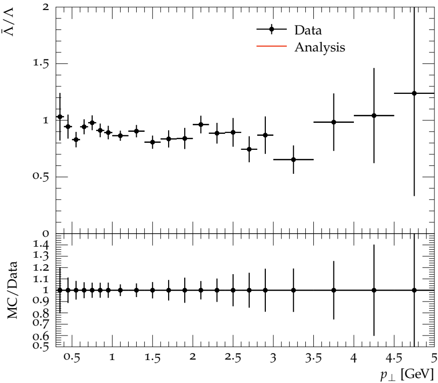
Ratio of \bar{\Lambda}/\Lambda as function of p_{\perp}
