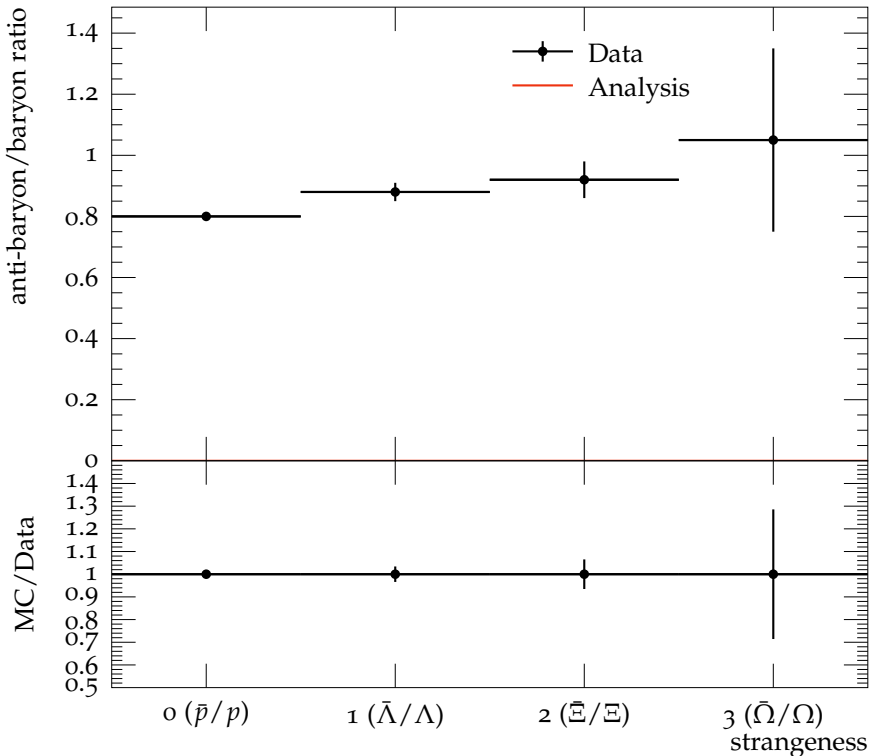
Anti-baryon over baryon ratio vs strangeness
