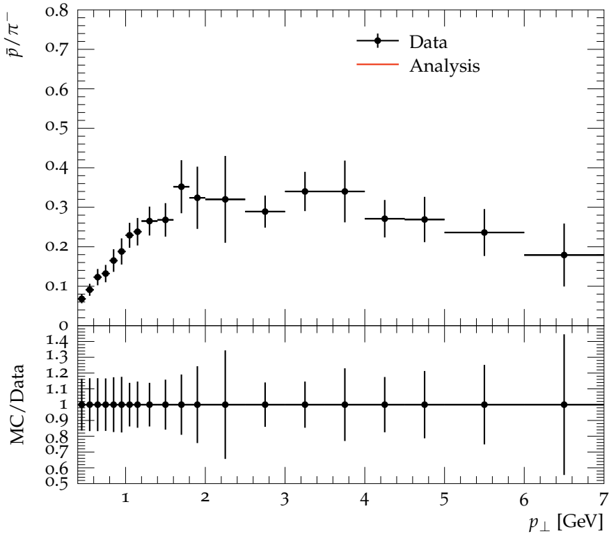
Ratio of \bar{p}/\pi^- as function of p_{\perp}
