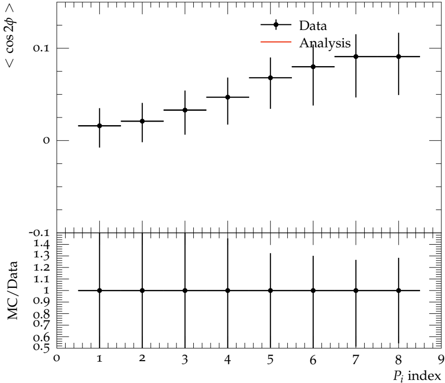
Average \cos 2\phi vrs P_i : 0.25, 0.5, 0.75, 1.0, 1.25, 1.5, 1.75, 2.0 GeV
