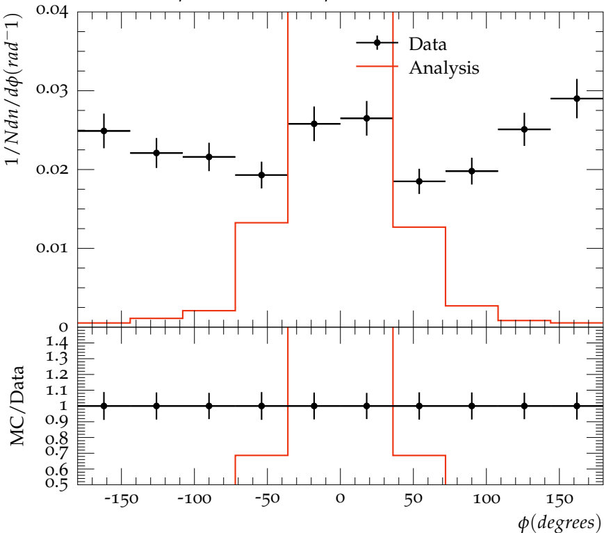
Differential \phi distribution for p_T = 2 GeV
