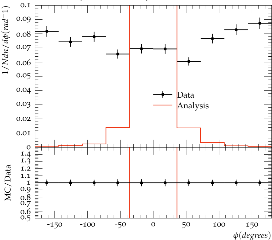
Differential \phi distribution for p_T = 0.5 GeV
