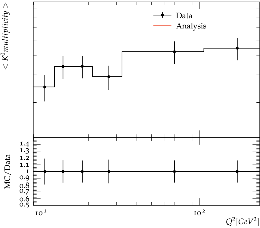
Mean multiplicity of K^0 vs. Q^2
