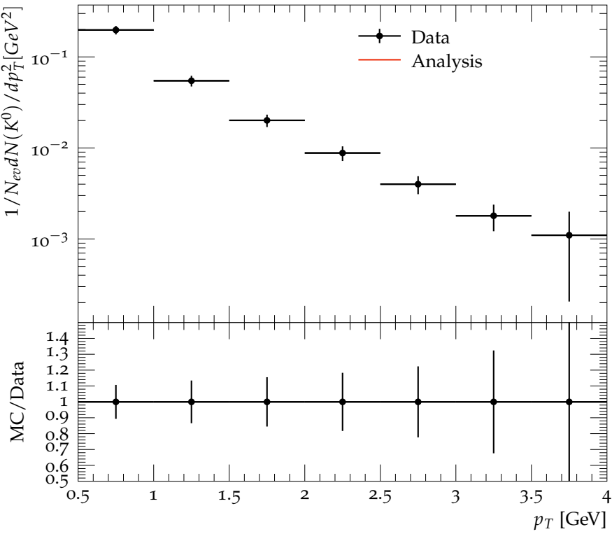
Differential multiplicity of K^0 vs. p_T
