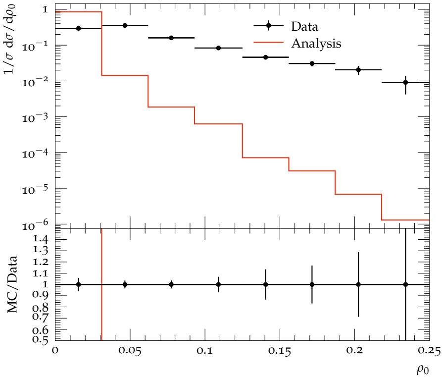
\rho_0 distribution for \langle Q \rangle = 24\text{GeV}
