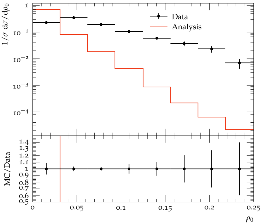
\rho_0 distribution for \langle Q \rangle = 18\text{GeV}
