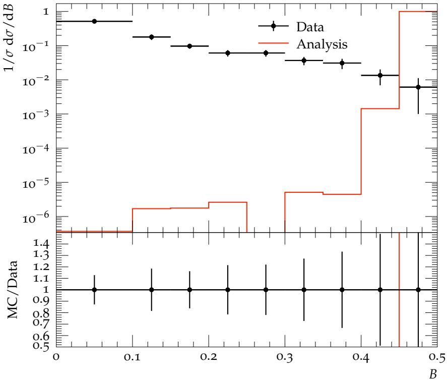
B distribution for \langle Q \rangle \geq 81\text{GeV}
