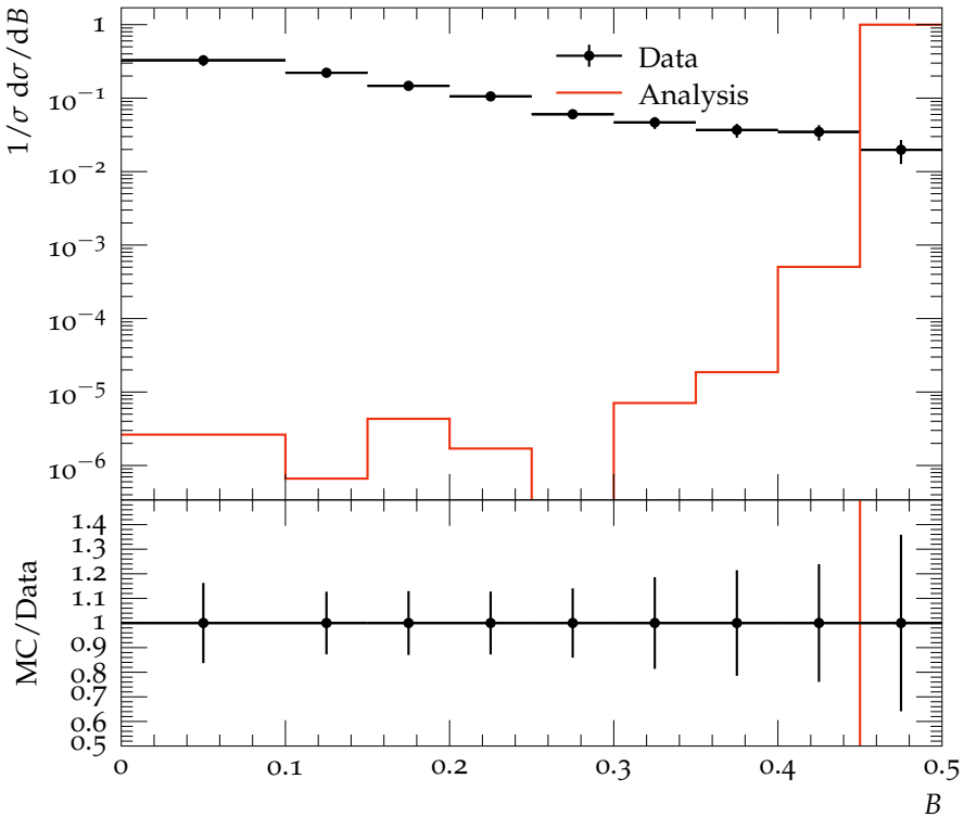
B distribution for \langle Q \rangle \leq 58\text{GeV}
