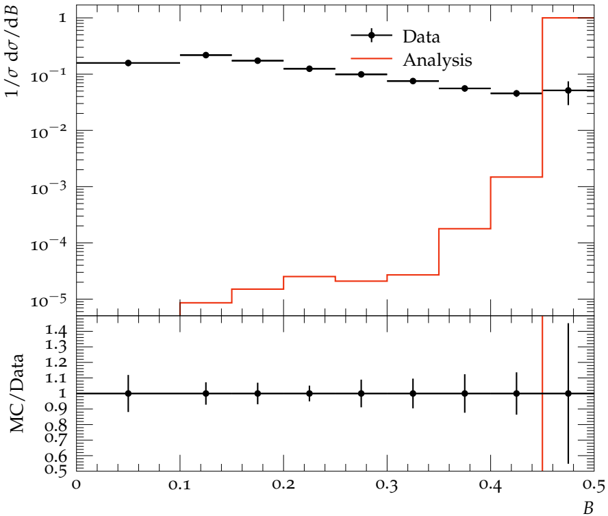
B distribution for \langle Q \rangle \geq 37\text{GeV}
