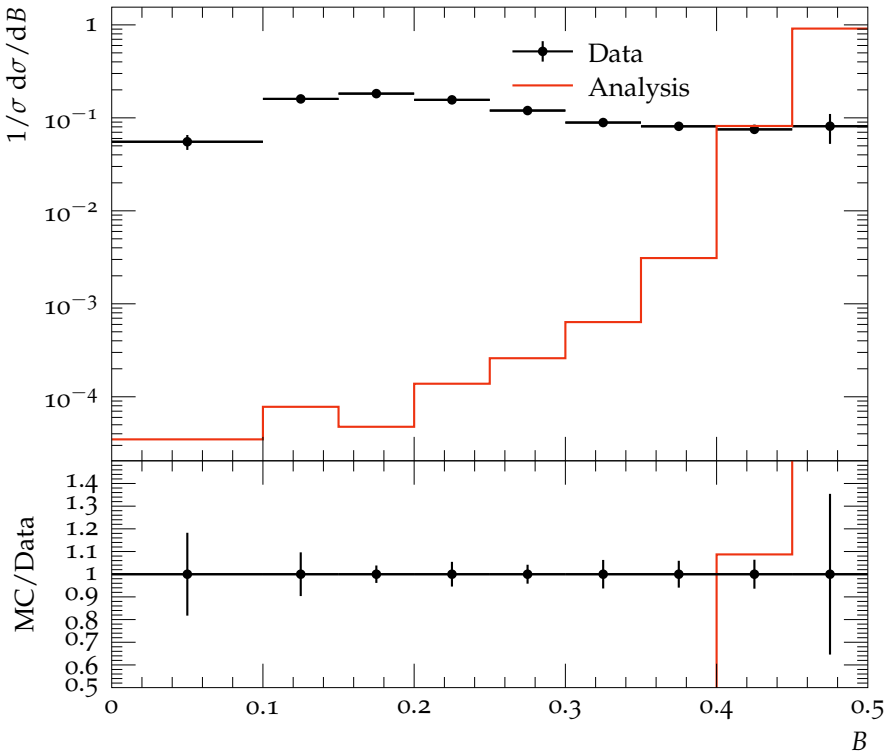
B distribution for \langle Q \rangle \leq 24\text{GeV}
