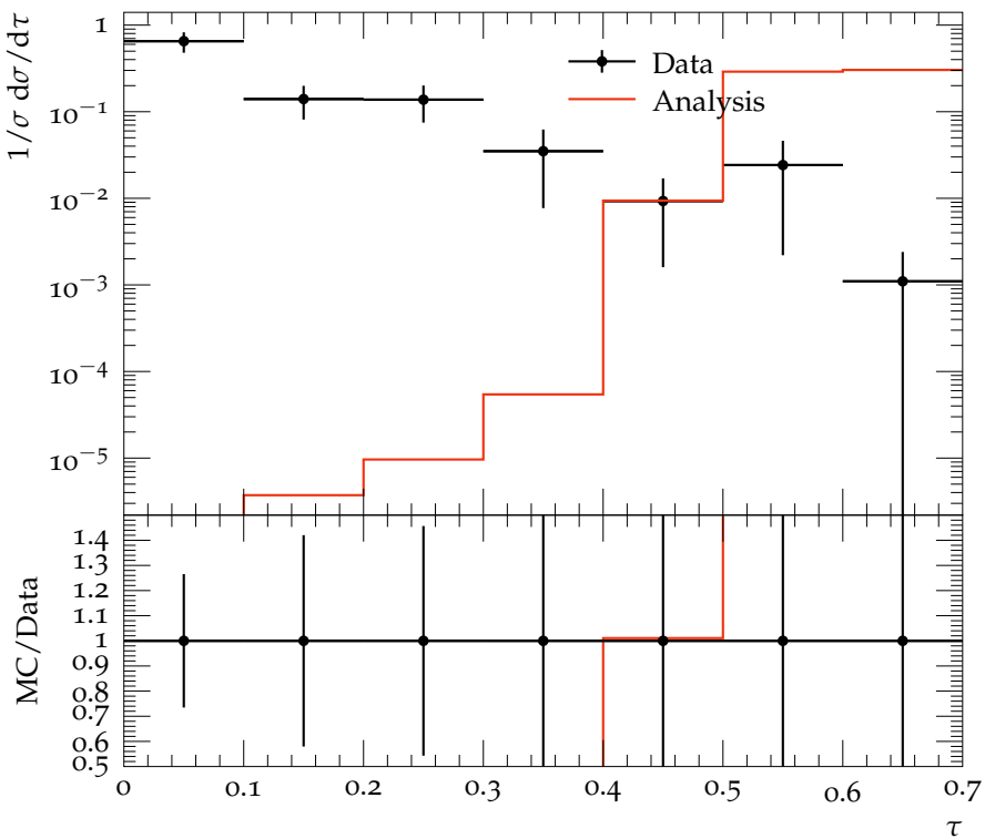
\tau distribution for \langle Q \rangle \leq 116\text{GeV}
