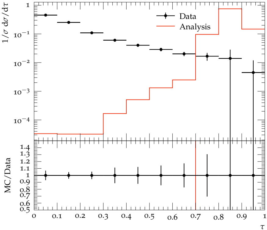
\tau distribution for \langle Q \rangle \geq 37\text{GeV}
