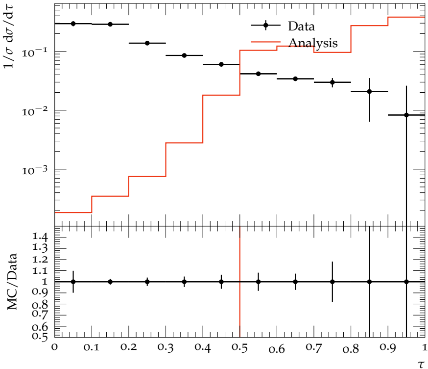
\tau distribution for \langle Q \rangle \geq 24\text{GeV}
