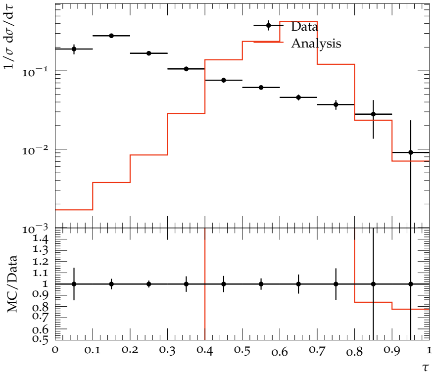
\tau distribution for \langle Q \rangle \leq 18\text{GeV}
