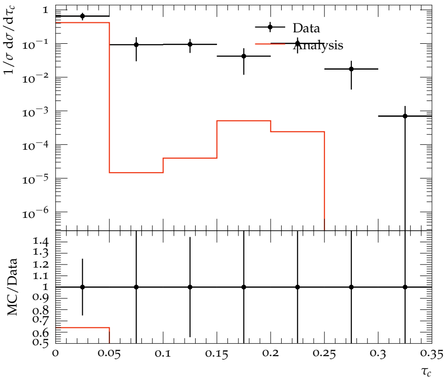
\tau_c distribution for \langle Q \rangle = 116\text{GeV}
