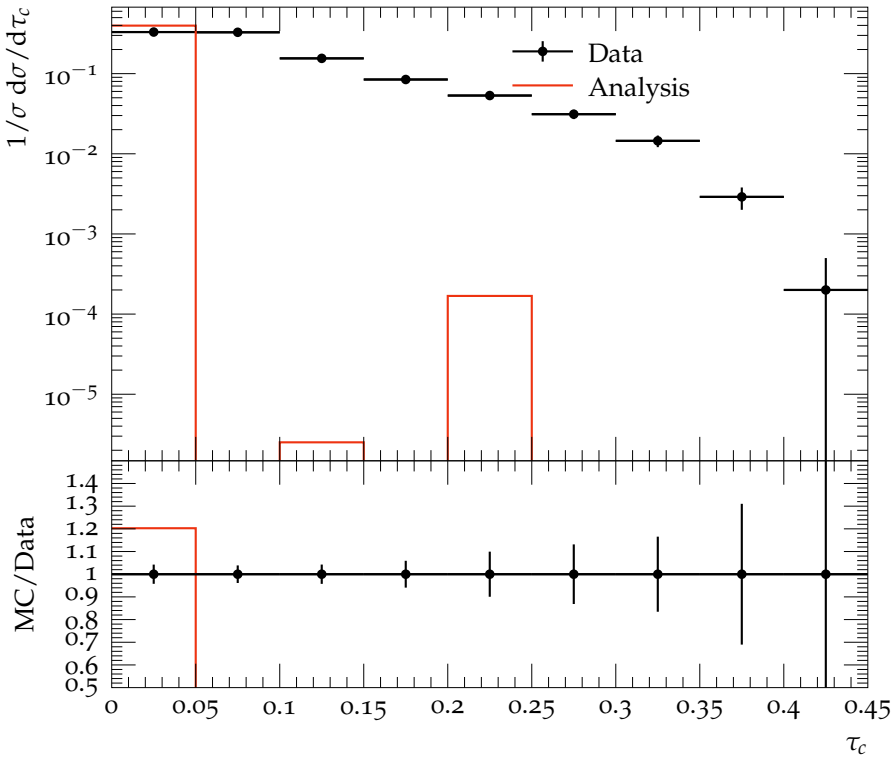
\tau_c distribution for \langle Q \rangle = 37\text{GeV}
