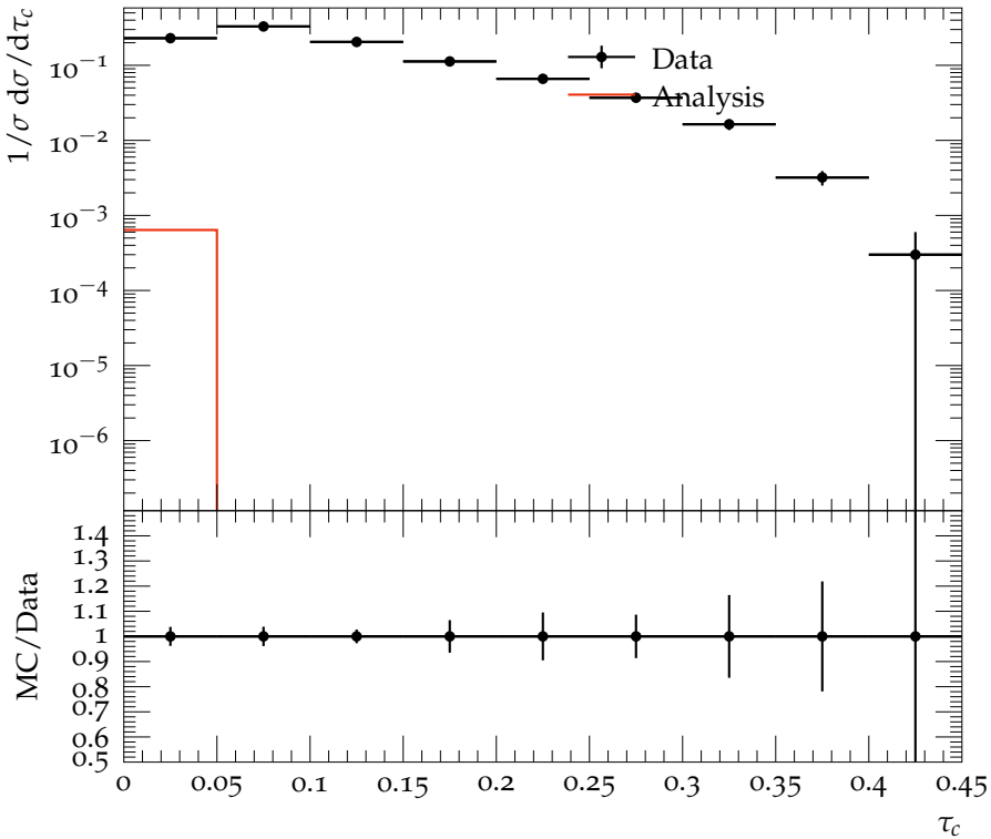
\tau_c distribution for \langle Q \rangle = 24\text{GeV}
