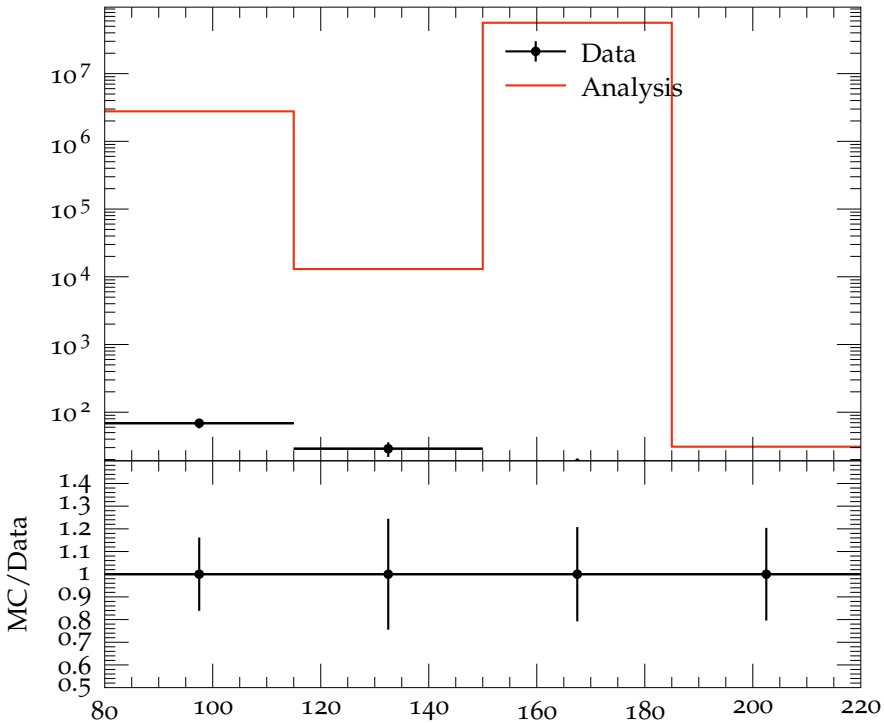
C_4 vs W , 4 < \eta < 5
