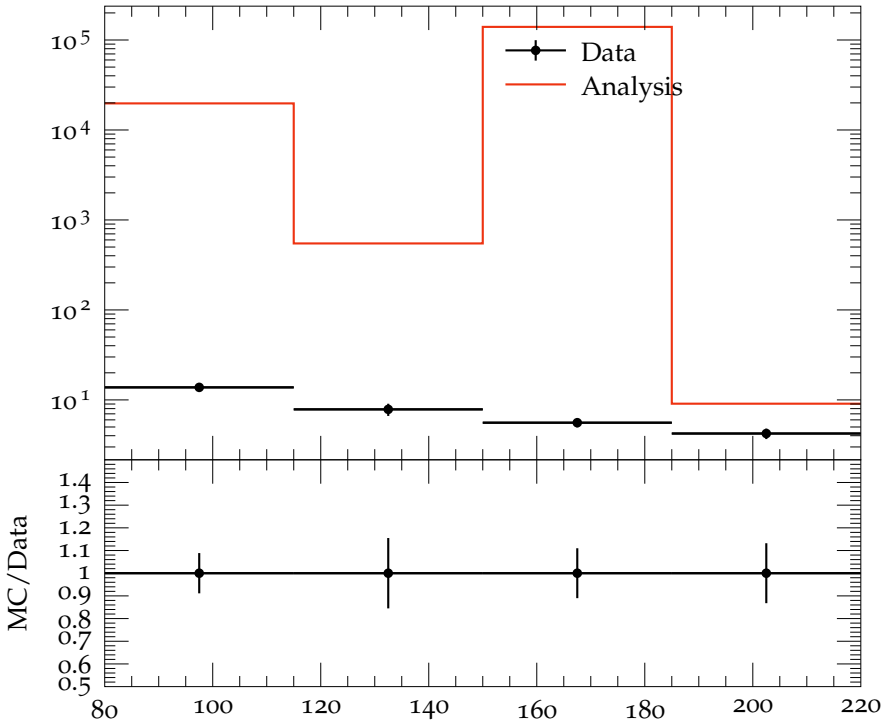
C_3 vs W , 4 < \eta < 5
