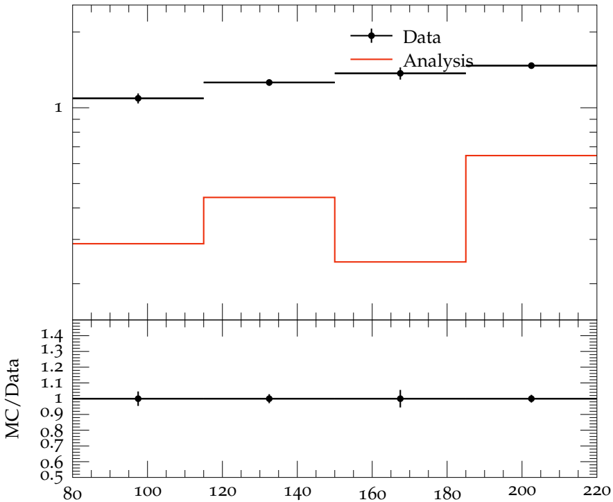
D_4 vs W , 4 < \eta < 5
