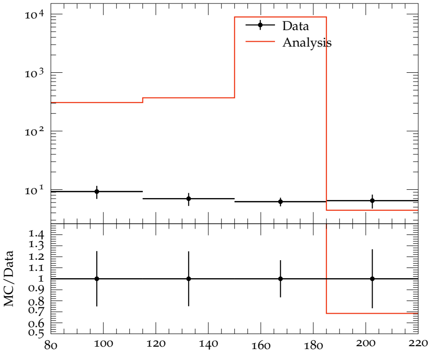
C_4 vs W , 3 < \eta < 4
