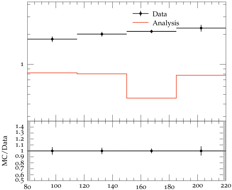
D_4 vs W , 3 < \eta < 4
