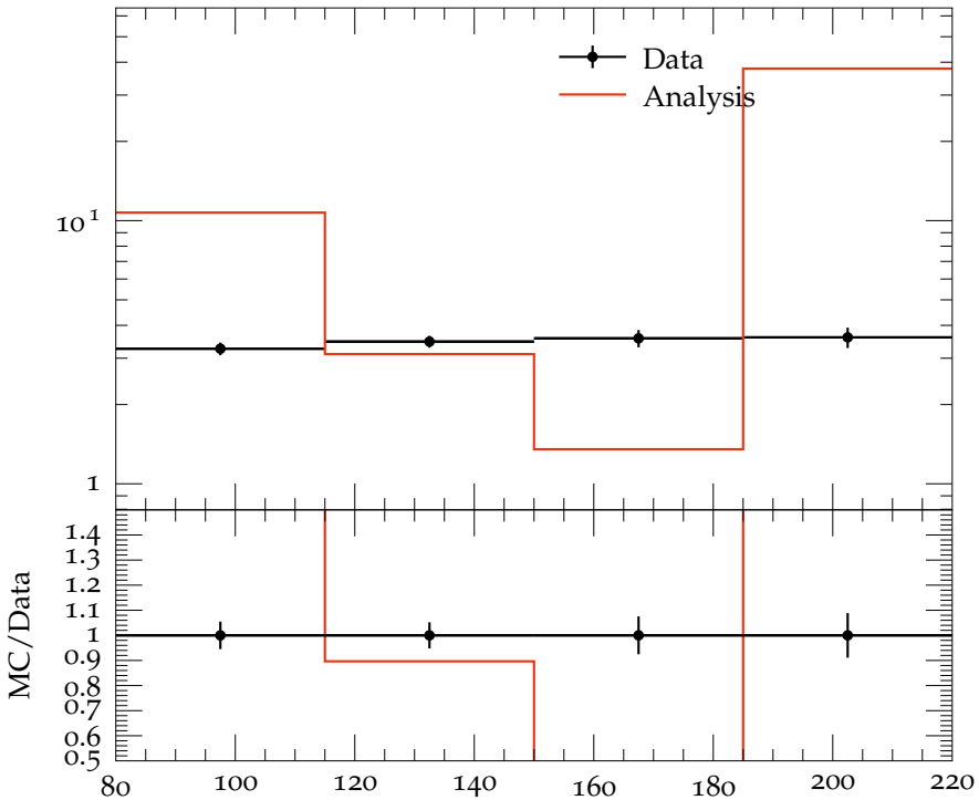
C_3 vs W , 2 < \eta < 3
