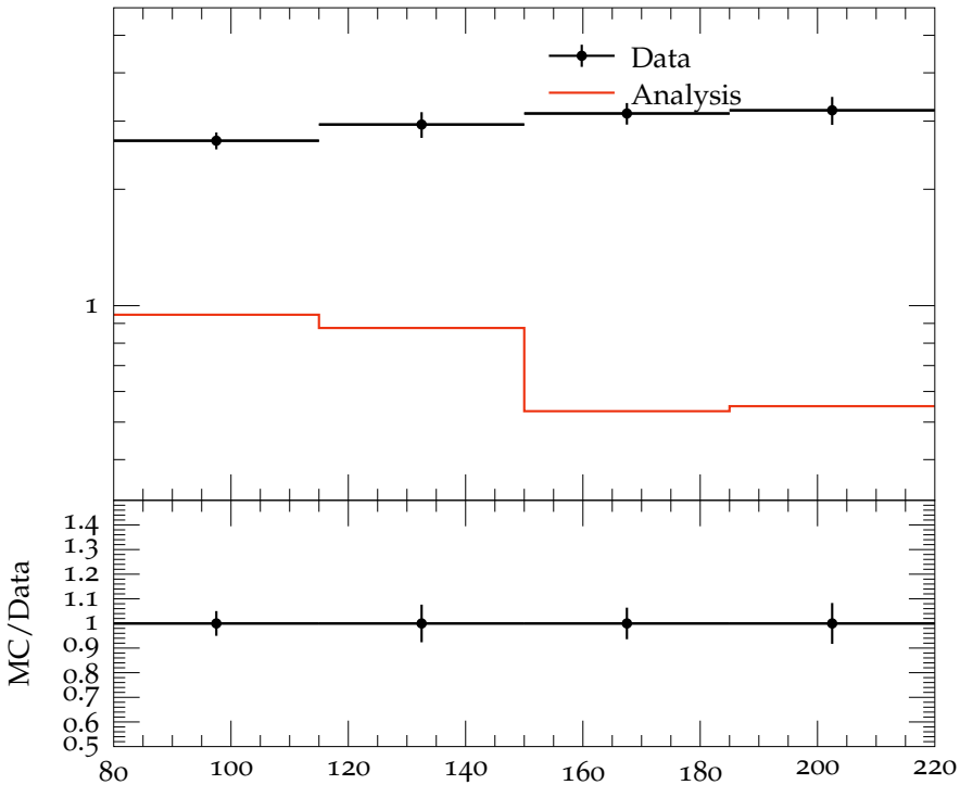
D_4 vs W , 2 < \eta < 3
