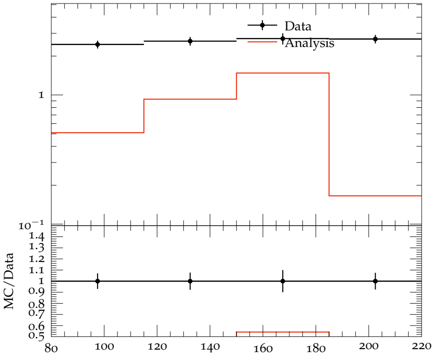
Mean multiplicity vs W , 2 < \eta < 3
