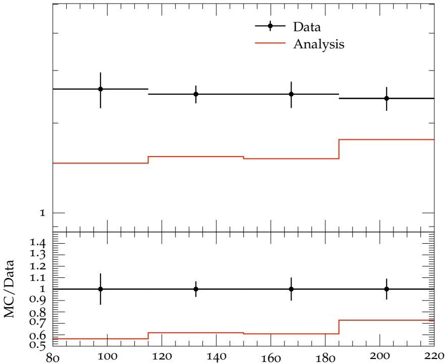
C_4 vs W , 1 < \eta < 5
