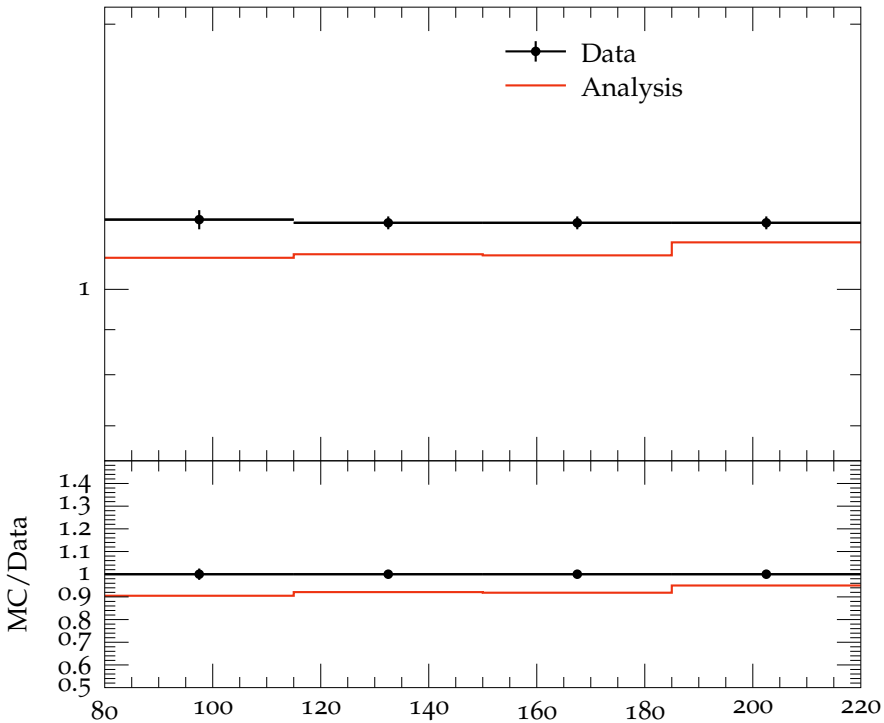
C_2 vs W , 1 < \eta < 5
