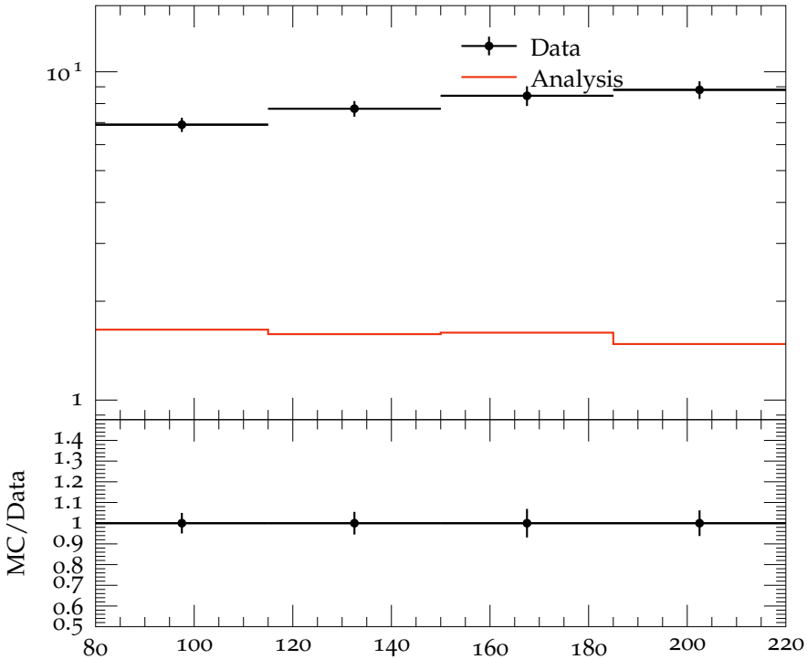
Mean multiplicity vs W , 1 < \eta < 5
