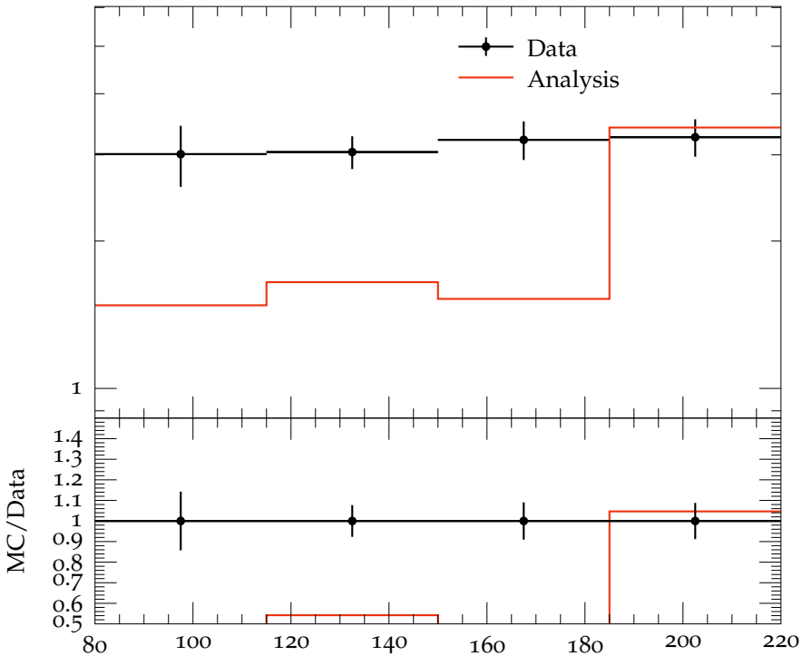
C_4 vs W , 1 < \eta < 4
