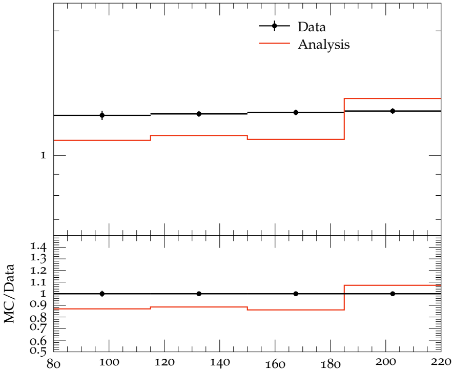
C_2 vs W , 1 < \eta < 4
