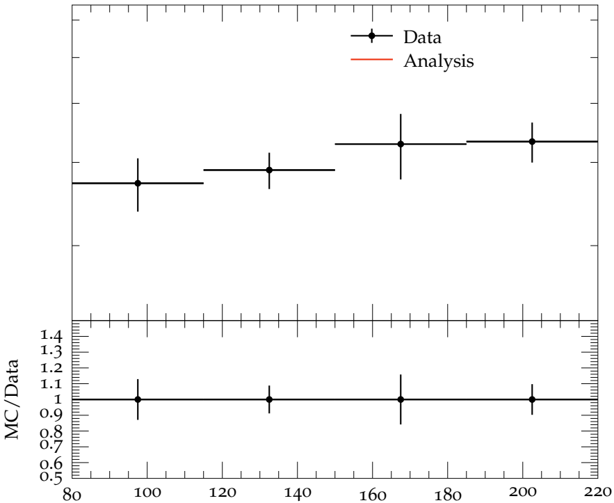
D_3 vs W , 1 < \eta < 4
