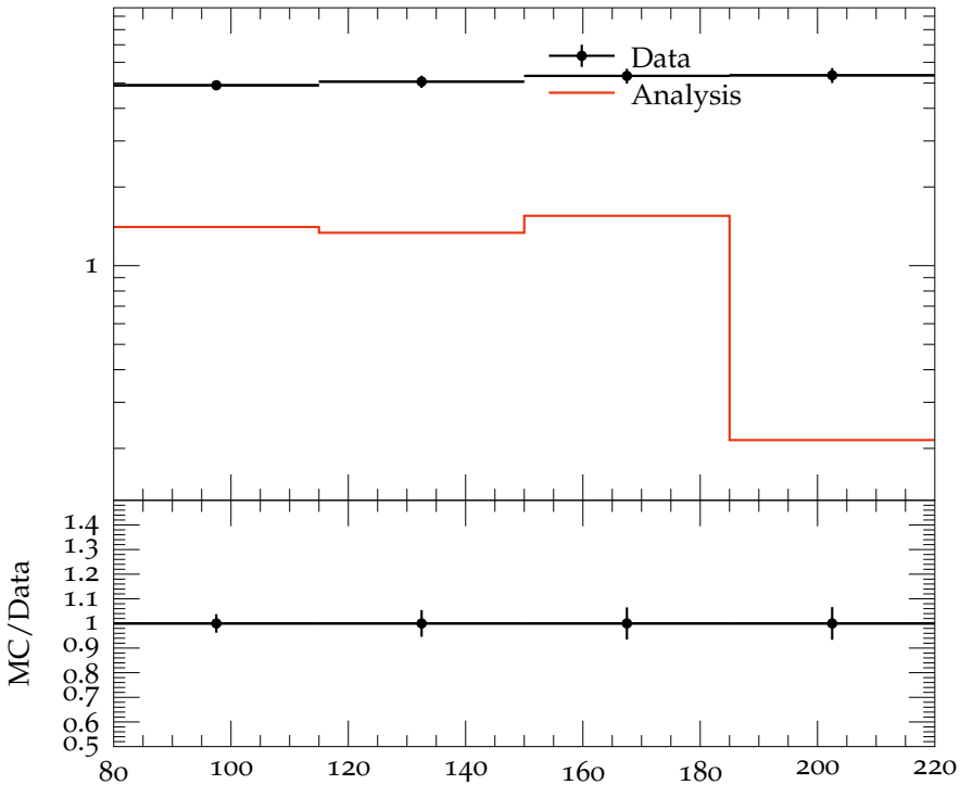
Mean multiplicity vs W , 1 < \eta < 3
