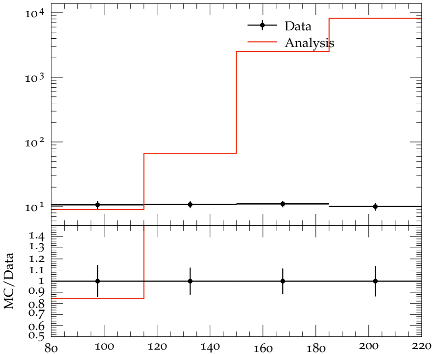
C_4 vs W , 1 < \eta < 2
