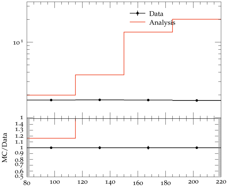
C_2 vs W , 1 < \eta < 2
