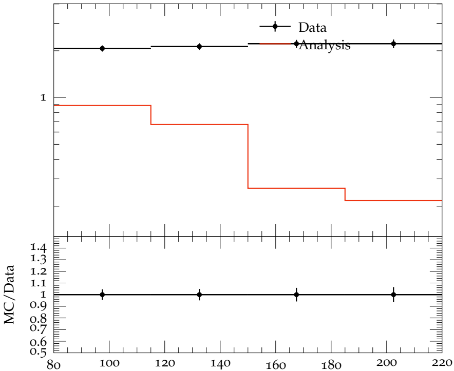
D_2 vs W , 1 < \eta < 2
