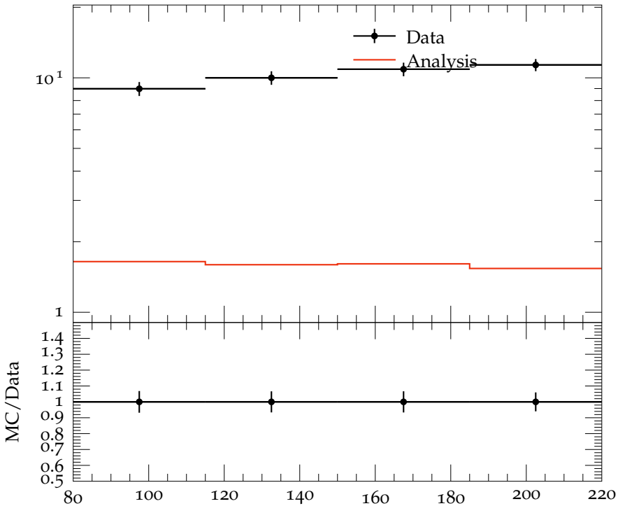
Mean multiplicity vs W , 0 < \eta
