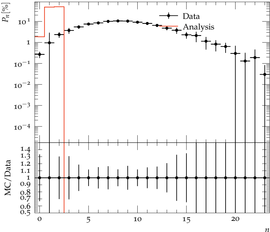
P_n vs multiplicity 1 < \eta < 5 , 185 < W < 220 GeV
