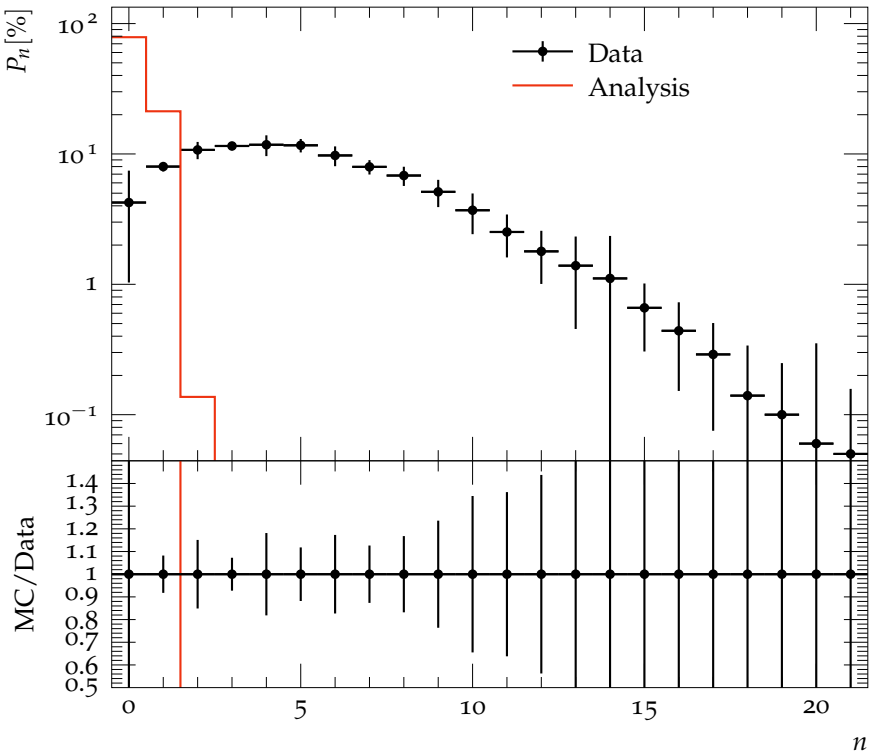
P_n vs multiplicity 1 < \eta < 3, 185 < W < 220 GeV
