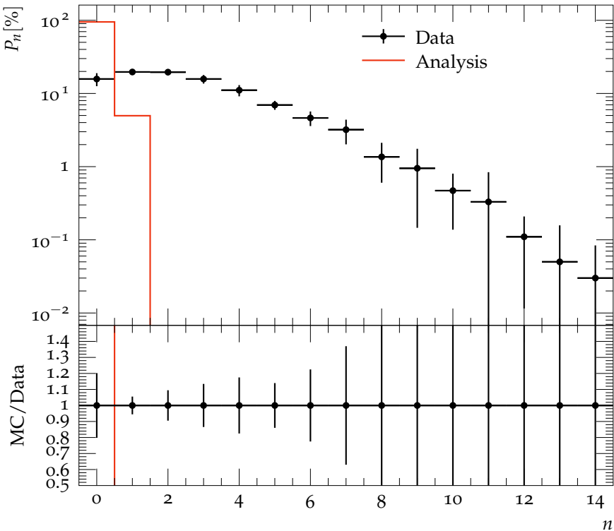
P_n vs multiplicity 1 < \eta < 2 , 185 < W < 220 GeV
