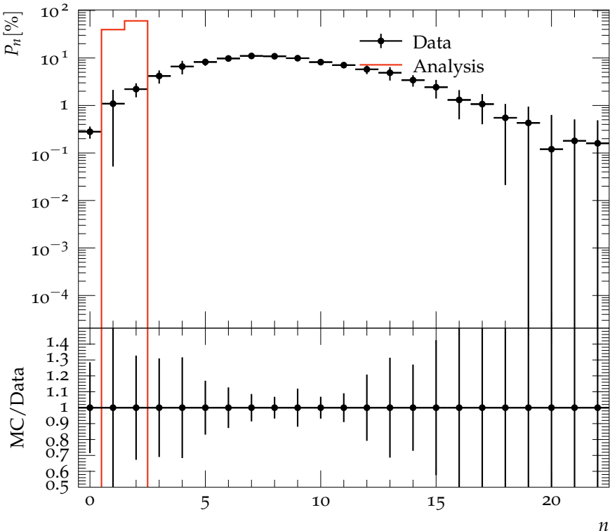
P_n vs multiplicity 1 < \eta < 5, 150 < W < 185 GeV
