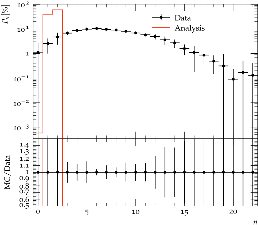
P_n vs multiplicity 1 < \eta < 4, 150 < W < 185 GeV
