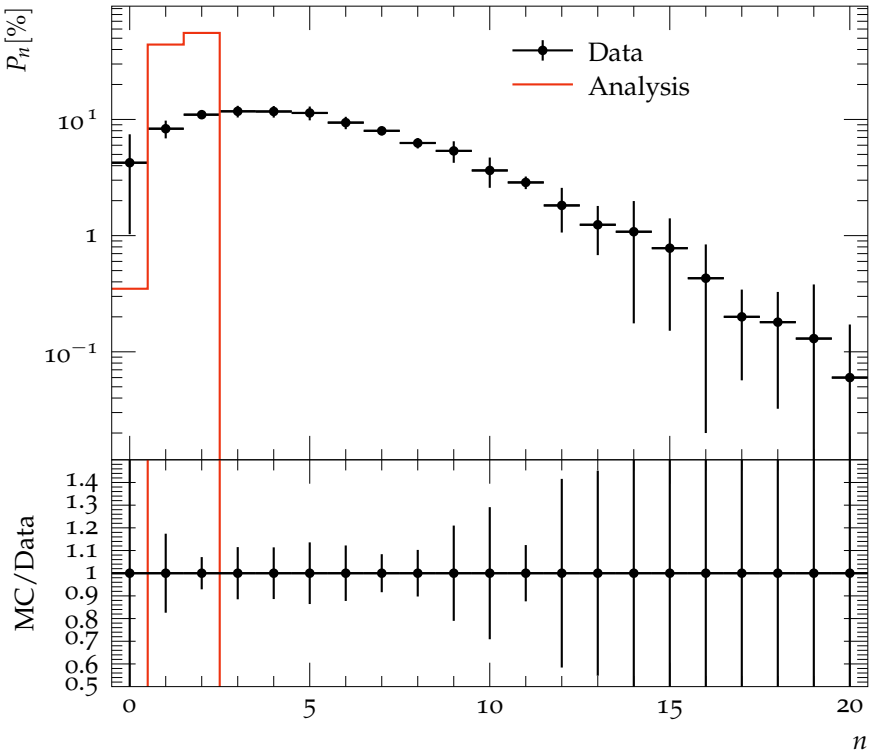
P_n vs multiplicity 1 < \eta < 3, 150 < W < 185 GeV
