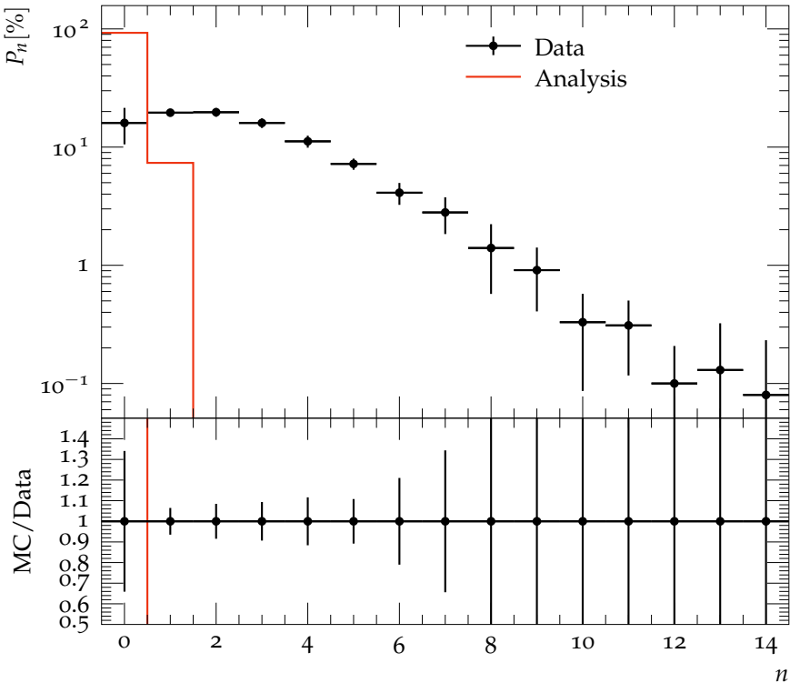
P_n vs multiplicity 1 < \eta < 2 , 150 < W < 185 GeV
