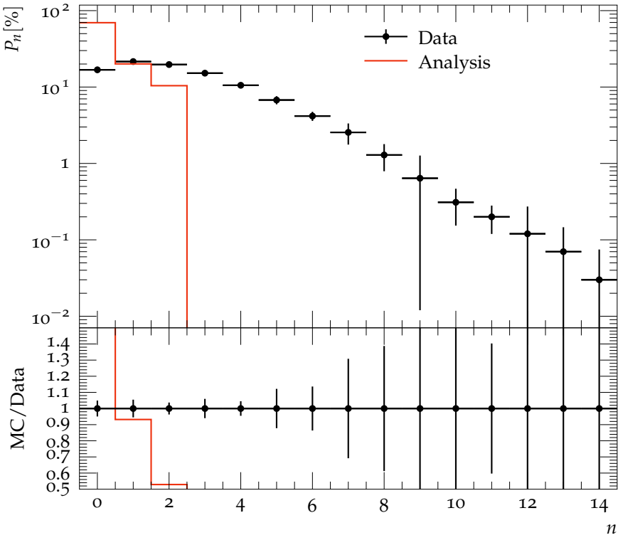
P_n vs multiplicity 1 < \eta < 2, 115 < W < 150 GeV
