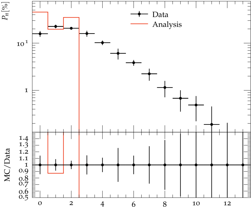
P_n vs multiplicity 1 < \eta < 2, 80 < W < 115 GeV
