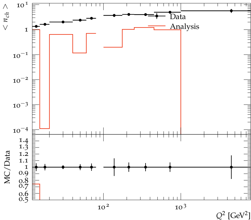
Average charged particle multiplicity vrs. Q^2
